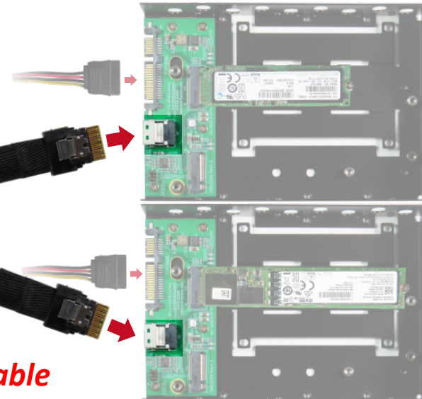
3.5" SlimSAS & SATA to M.2/M.3 NVMe SSD & M.2 SATA Drive Tray
