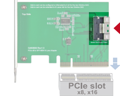
Model No.: PE0804 PCIe x8 to SlimSAS (SFF-8654) 8-Lane Adapter
