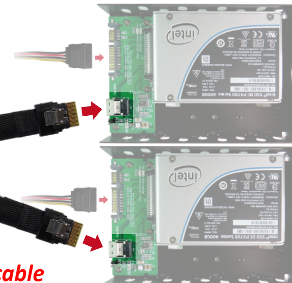
3.5" SlimSAS & SATA to U.2 / SAS / SATA SSD Adapter
